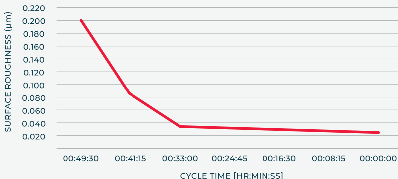
CYCLE TIME VS SURFACE FINISH
